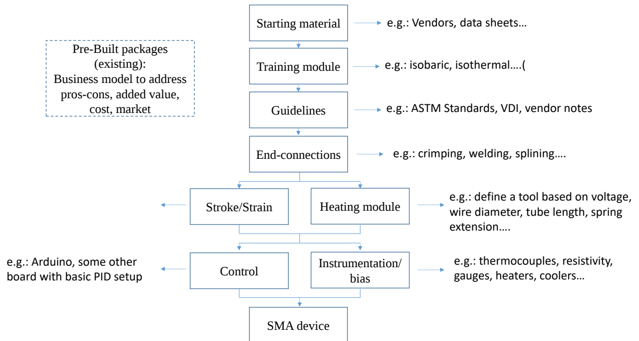
4. Figure A1: A flow chart showing an example of several modules required for designing an SMA actuator/device. (Not inclusive or generalized).
